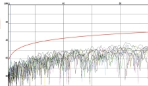
NEXT (MHz)
